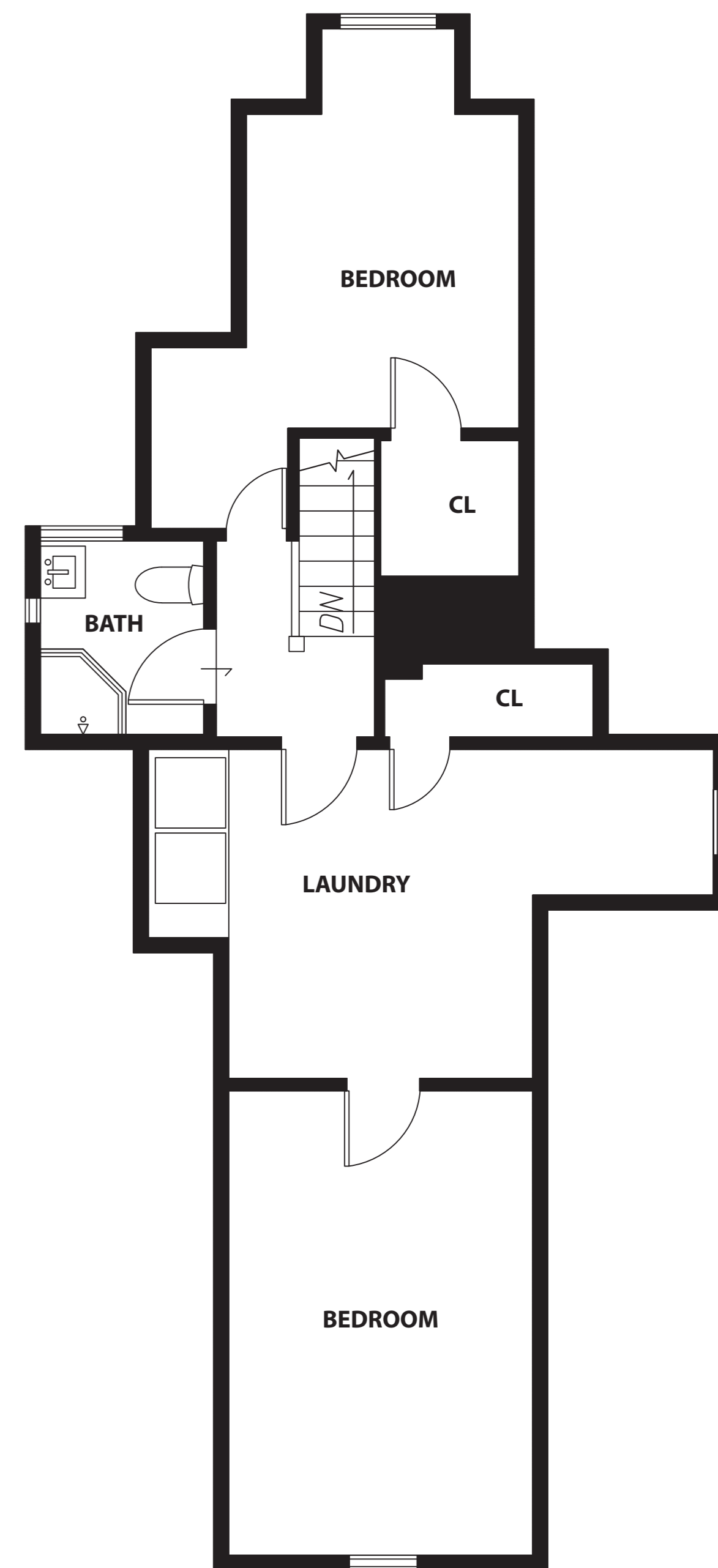
UNIT #3 (THIRD FLOOR)
